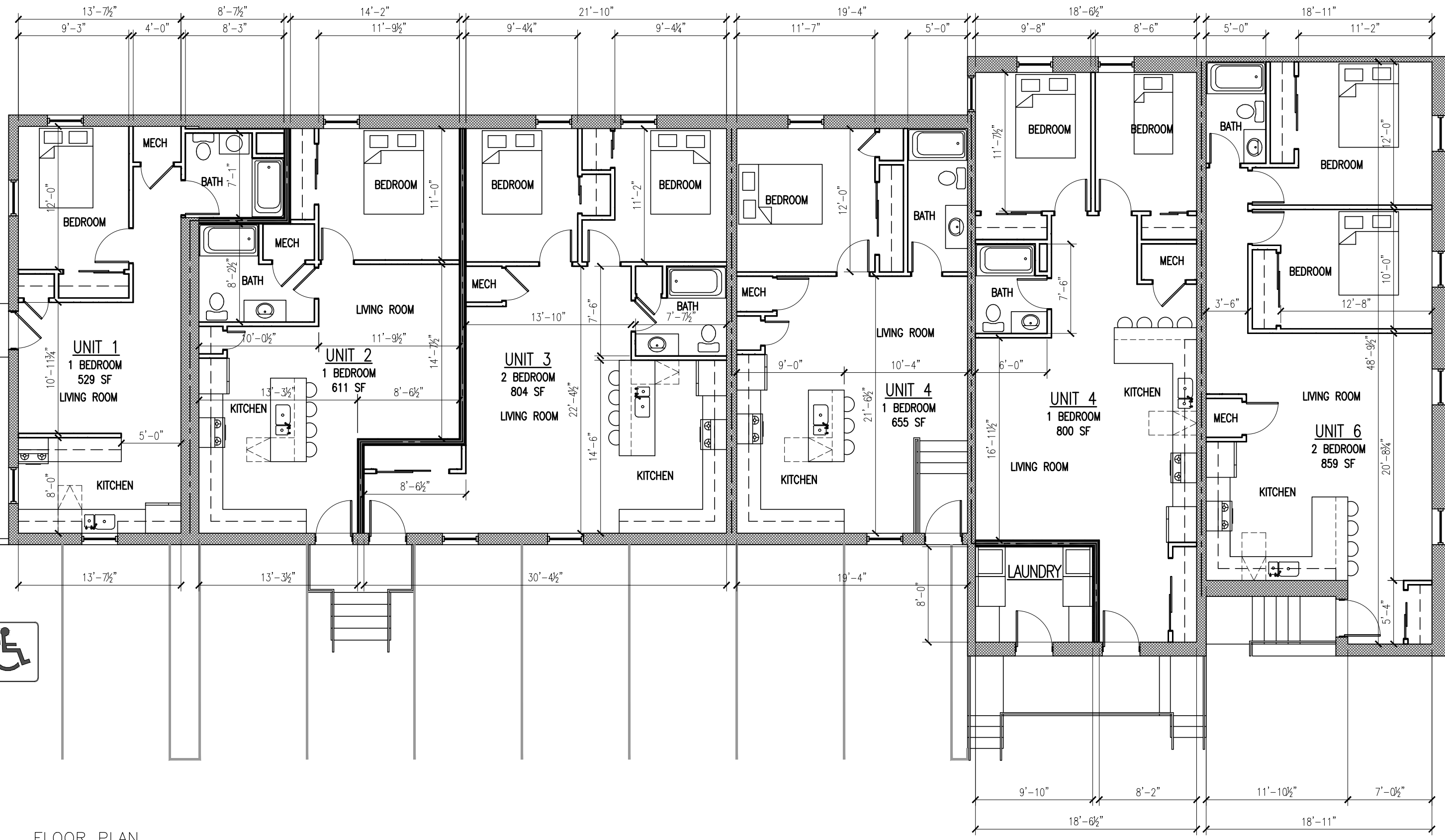
FLOOR PLAN 1/8" = 1'-0"
